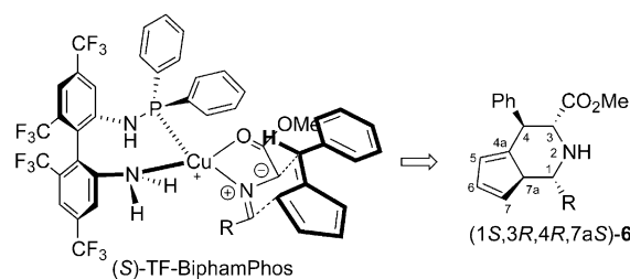
Figure 2. Proposed transition state leading to (1 S ,3 R ,4 R ,7 a S )- 6 .
